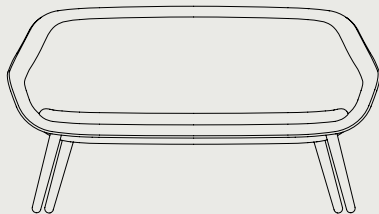
AAL SOFA W150 x D73 x H81/SH40 cm
